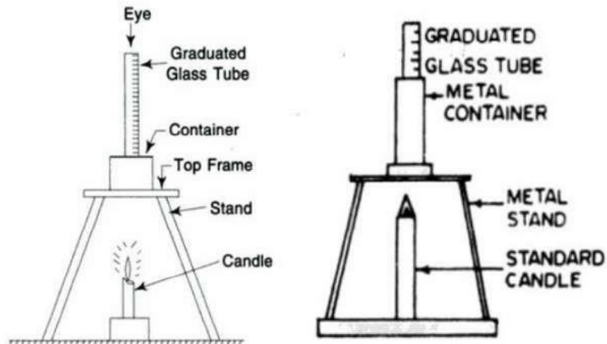
Jackson's Turbidimeter
