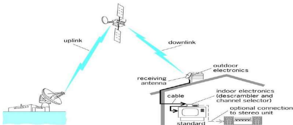
Direct broadcasting satellite system
