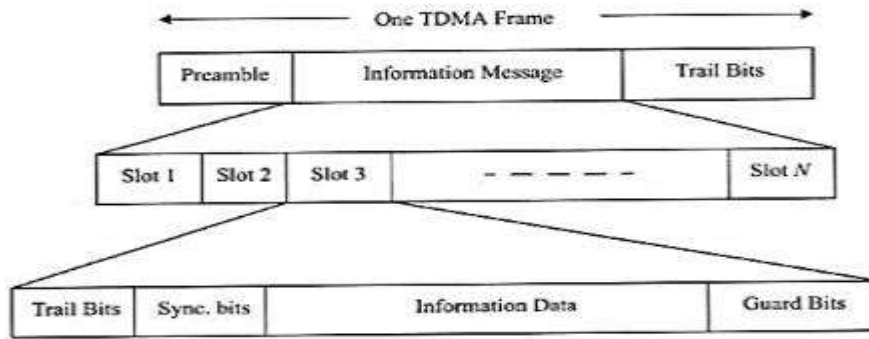
Fig: TDMA frame structure
