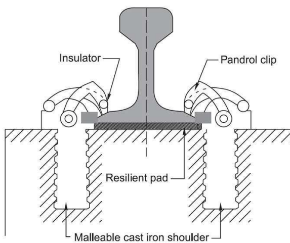
Insulated liners
