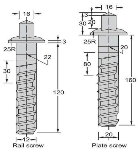
Screw spikes
