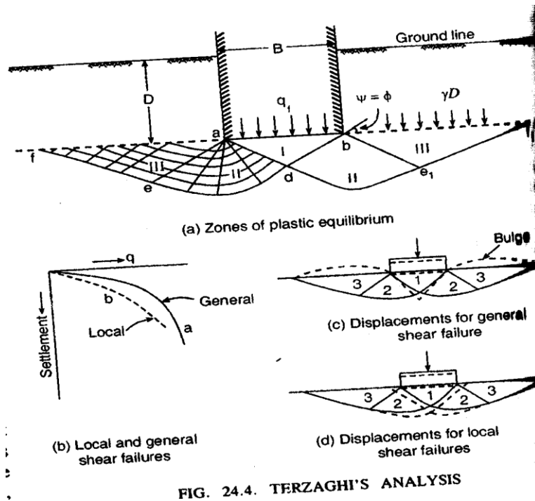
FIG. 9.4 TERZAGHI'S ANALYSIS
