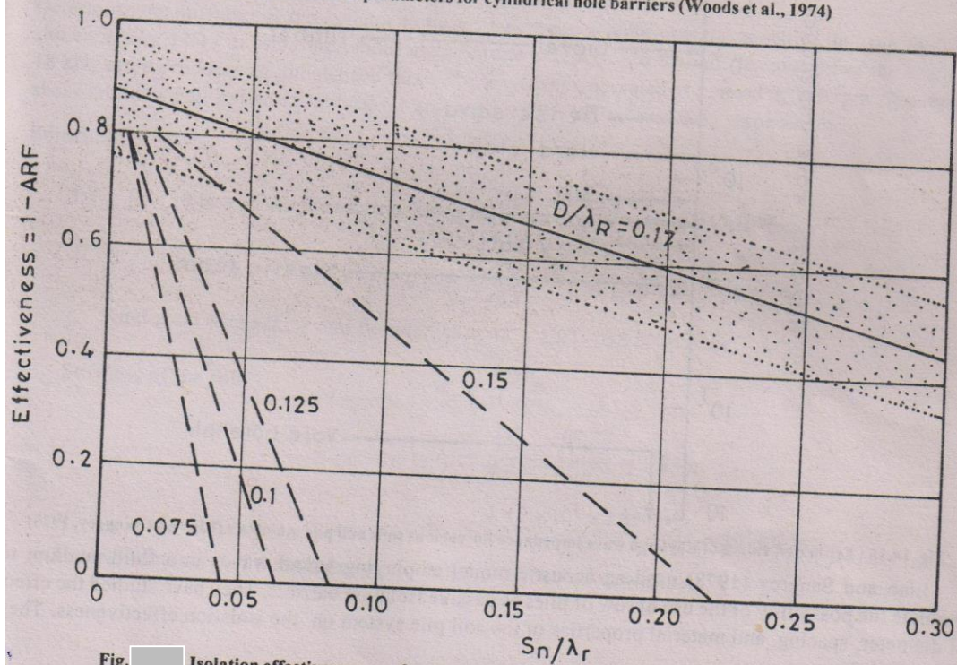
Fig. 14.15 Isolation effectiveness as a function of hole diameter and spacing (Woods et al., 1974)
