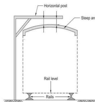
Fig. 2.2 Loading gauge
