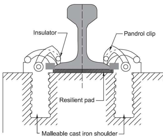
Insulated liners
